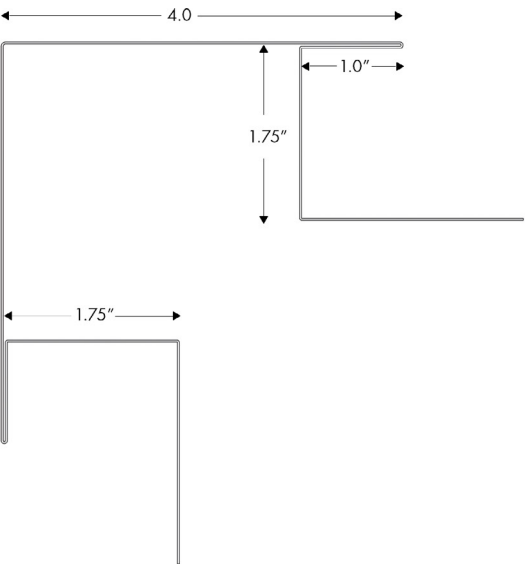
Corner Post 900204
