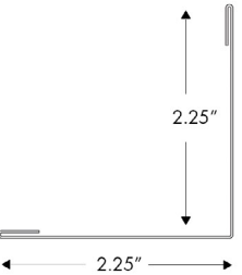
Outside L Trim 900200
