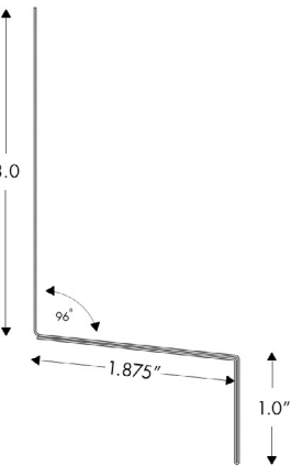
Belt Line / Window Flashing 900110
