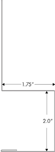
Box Base 900116
