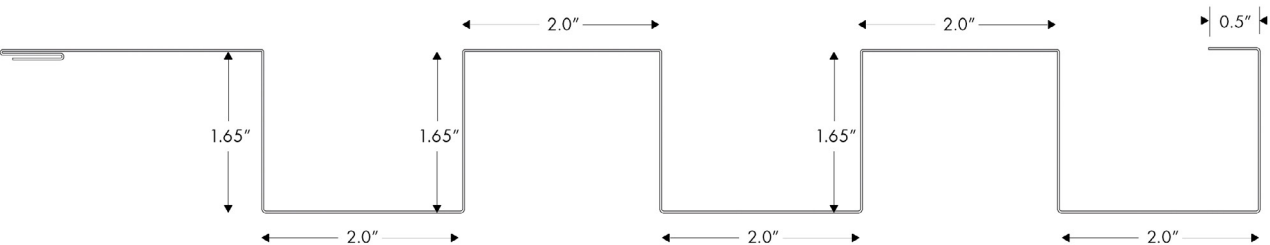
Folded Wall ( 20' - 900104 / 13' - 900102 / 10' - 900100 )
