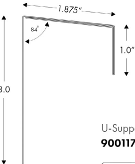
Reverse Window Flashing 900118
