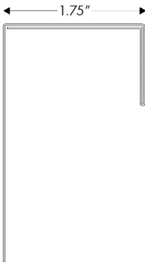
One Piece J-Trim 900112
