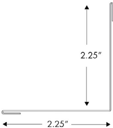
Inside L Trim 900202
