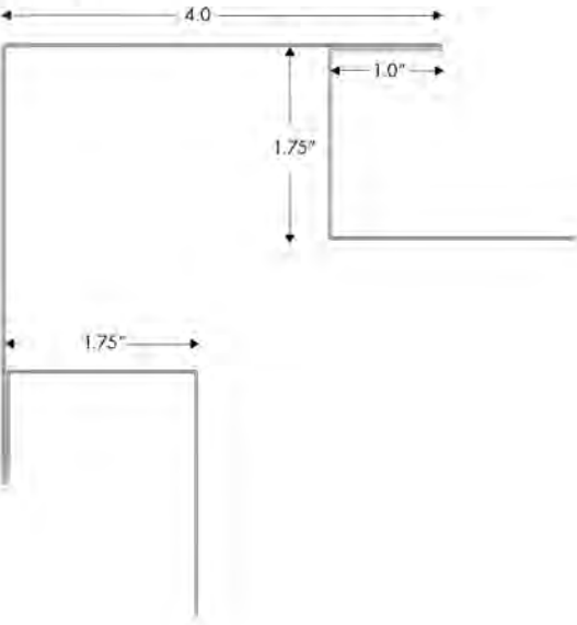
Corner Post 900204
