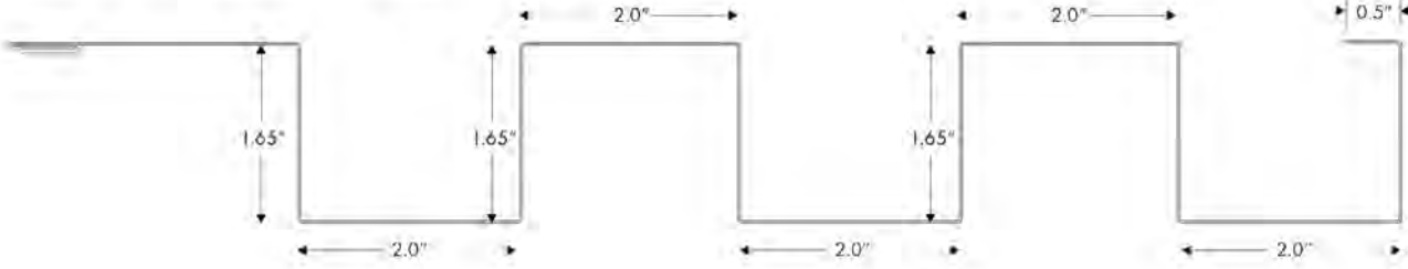
Folded Wall ( 20' - 900104 / 13' - 900102 / 10' - 900100 )
