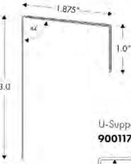
Reverse Window Flashing 900118
